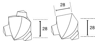
CONECTORES ÁNGULO INTERIOR REF. 3 CONNECTING PIECES FOR THE INSIDE ANGLE PROFILE REF. 3
