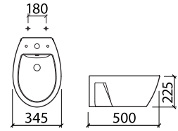
131455 bidé suspenso com furo para tampo wall hung bidet w/ holes f/ cover bidet suspendu a/ trous p/ abattant
