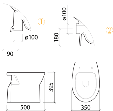
131012 ② sanita simples D/P W/D low-level wc cuvette simples S/H
