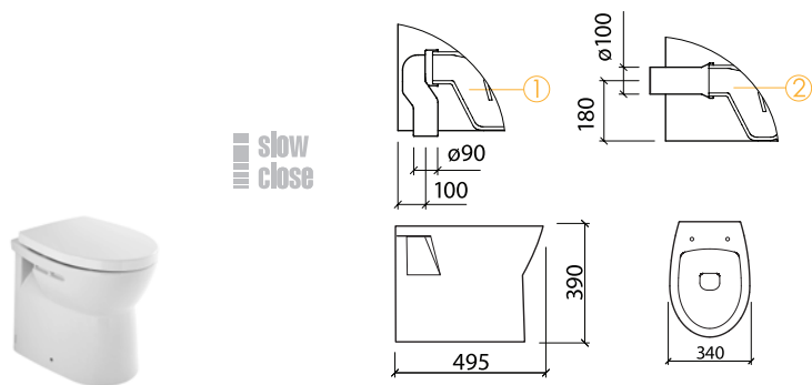
131013 ① sanita simples D/C wc fully enclosed F/D cuvette simple S/V
