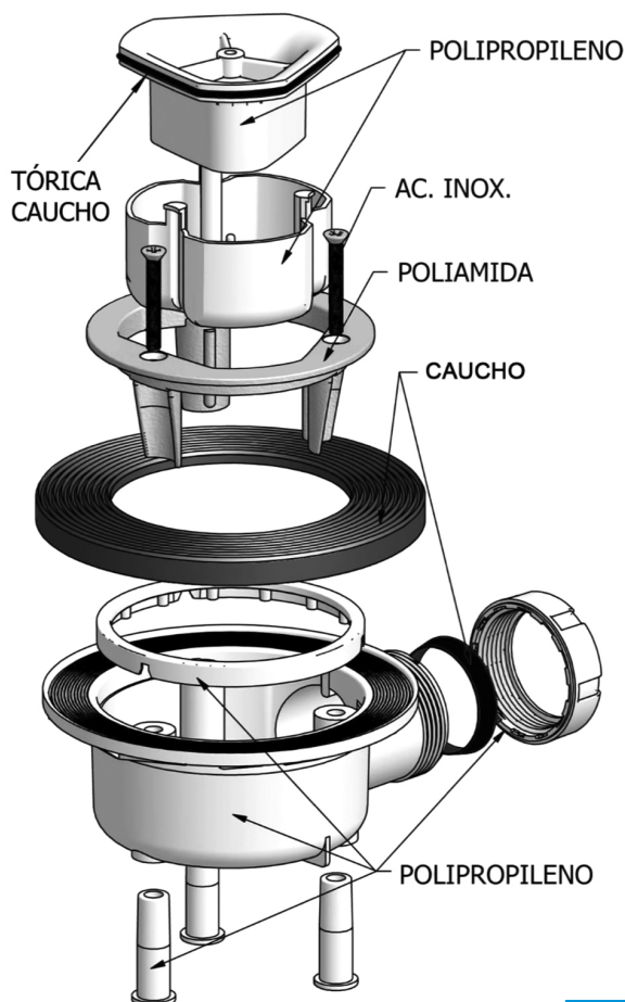
DESPIECE
