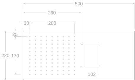
RCRK 99Z300708 Rociador de pared efecto lluvia y cascada Wall mounted rainshower and waterfall effect showerhead
