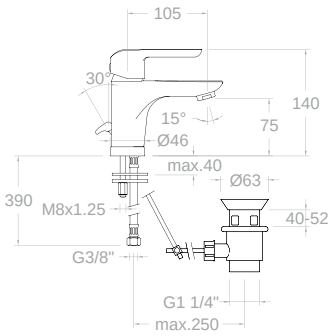
6601VA9065 261603 Monomando para lavabo con válvula automática 1 1/4 ". Ref. 9065 ABS Wash Basin mixer with pop-up waste 1 1/4 ". Ref. 9065 ABS
