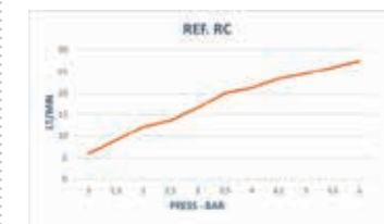
RCEXT 99Z303345 Rociador de cascada empotrado. Para exterior. Acabado cepillado mate Waterfall wall mounted shower. Outdoor. Finished brushed matte
