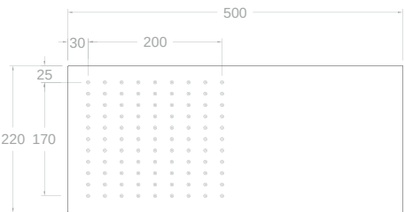
RRK 99Z300709 Rociador de pared efecto lluvia Wall mounted rainshower and effect showerhead
