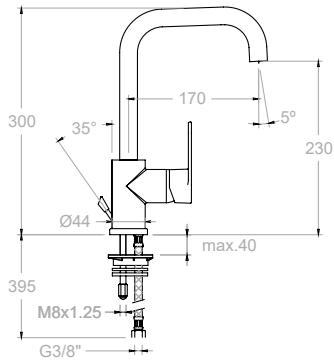
360302VA9065 36B303690 Monomando lavabo (S) con válvula automática 1 1/4" Ref. 9065 ABS. High wash basin mixer (S) with pop-up wate 1 1/4" Ref: 9065ABS
