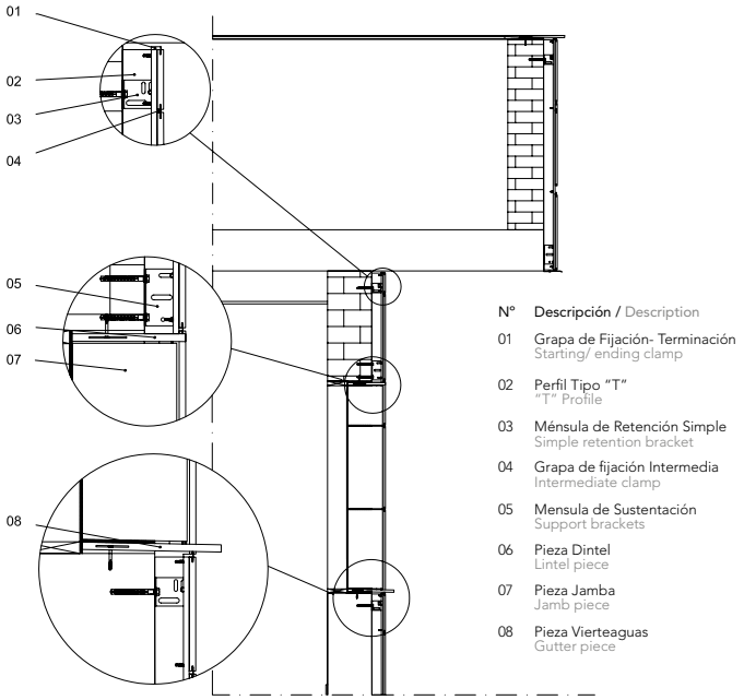
Componentes de aluminio / Aluminium components
