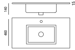
Lavabo SQUARE 1010 x 15 x 460 mm
