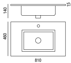
Lavabo SQUARE 810 x 15 x 460 mm
