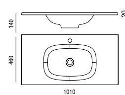
Lavabo BARI 1010 x 20 x 460 mm
