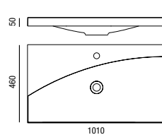
Basin AMALFI 1010 x 50 x 460 mm
