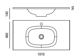
Basin BARI 1010 x 20 x 460 mm
