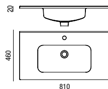
Basin MONZA 810 x 20 x 460 mm
