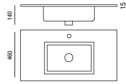
Basin SQUARE 1010 x 15 x 460 mm
