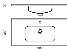
Basin MONZA 1010 x 20 x 460 mm
