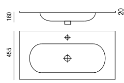
Basin NAPOLI 1010 x 20 x 455 mm
