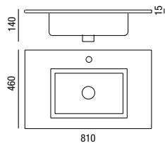
Basin SQUARE 810 x 15 x 460 mm
