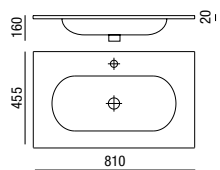
Basin NAPOLI 810 x 20 x 455 mm
