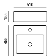
Basin on top PARMA 510 x 155 x 455
