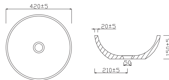
Lavabo Stella / Stella Washbasin
