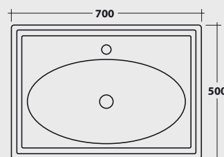
MELAMAJ70 Lavabo porcelana "MAJERLING-70" blanco MARJELING ceramic washbasin
