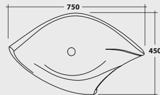
MELALKS75 Lavabo porcelana "LIKOS-75" blanco LIKOS ceramic washbasin
