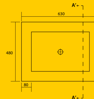
VACAL Lavabo Stonacril "CALCARE" CALCARE stonacril washbasin
