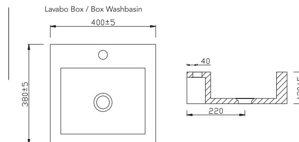
MABOX40 Lavabo stonacril mod. BOX BOX stonacril washbasin
